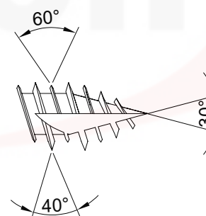
DETAIL C (1:2)
