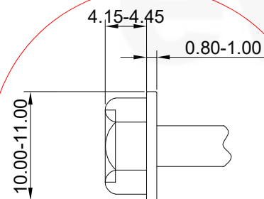
DETAIL A (1:2)
