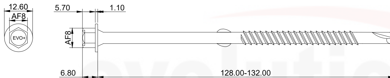
SSDH6.3-130-3
