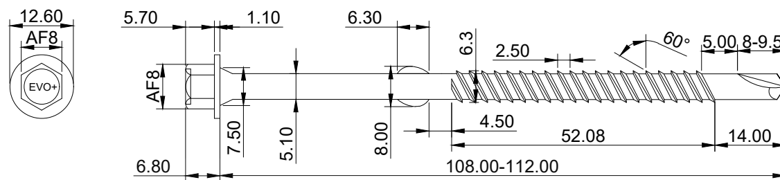
SSDH6.3-110-3
