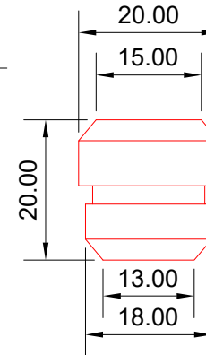
Washer Detail Scale 1:1
