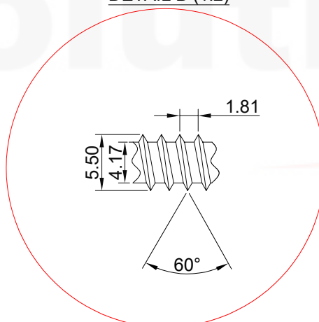
DETAIL B (1:2)
