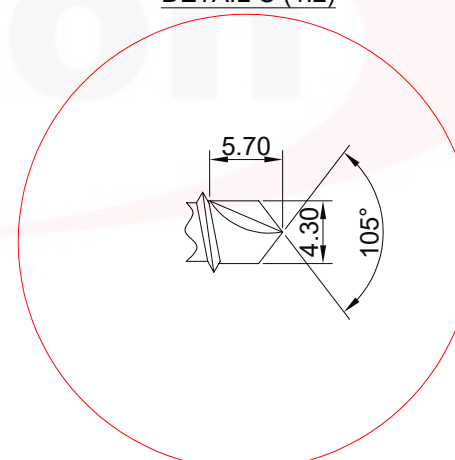
DETAIL C (1:2)
