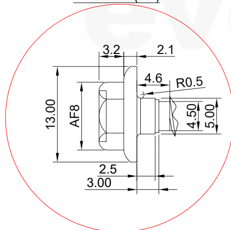
DETAIL A (1:2)
