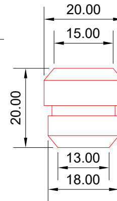
Washer Detail Scale 1:1
