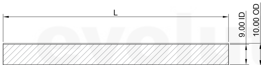
SSCS (STAINLESS STEEL COMPRESSION SLEEVE)
